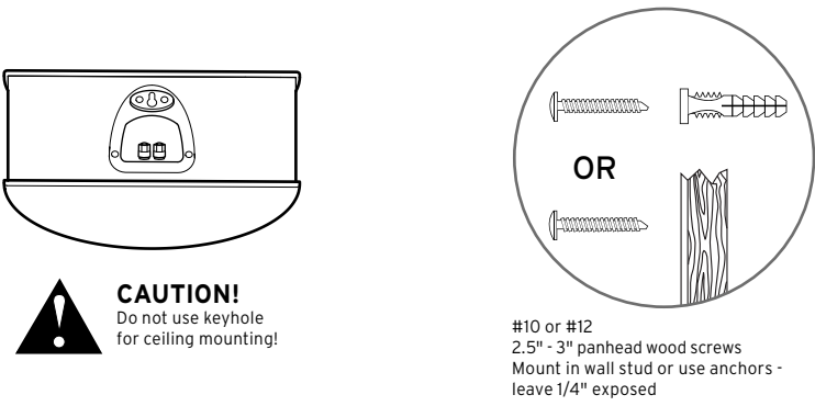
FIGURE 4 WALL MOUNTING SURROUND SPEAKERS
